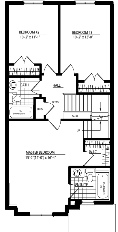
SECOND FLOOR PLAN 'A' 85 sq.ft. NOT INCLUDING 7 sq.ft. OPEN SPACE
