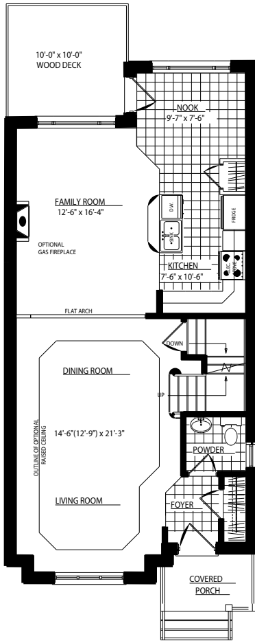
GROUND FLOOR PLAN 'A' 920 sq.ft.
