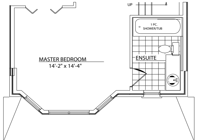
SECOND FLOOR PLAN 'C' 827 sq.ft.
