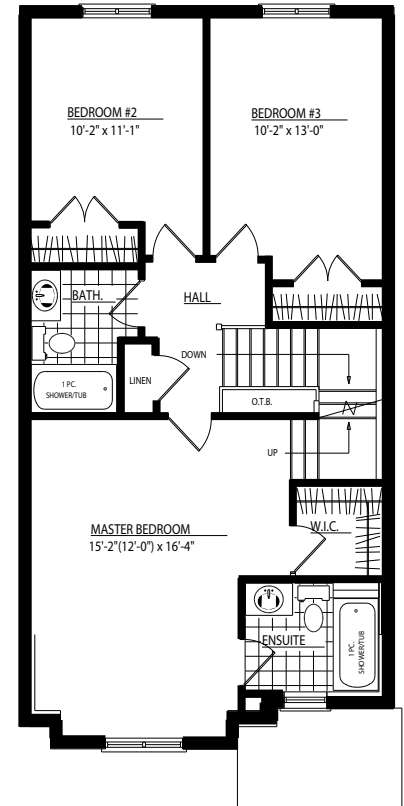
SECOND FLOOR PLAN 'A' 855 sq.ft.
